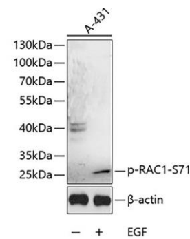
Fig. 1. Western blot analysis of extracts of A-431 cells, using Phospho-RAC1-S71 antibody at 1:1000 dilution. A431 cells were treated by EGF for 30 minutes after serum-starvation overnight. Secondary antibody: HRP-labeled Goat Anti-Rabbit IgG(H+L) (A0208) at 1:1000 dilution. Lysates/proteins: 25ug per lane. Blocking buffer: QuickBlock™ Blocking Buffer (P0231).
